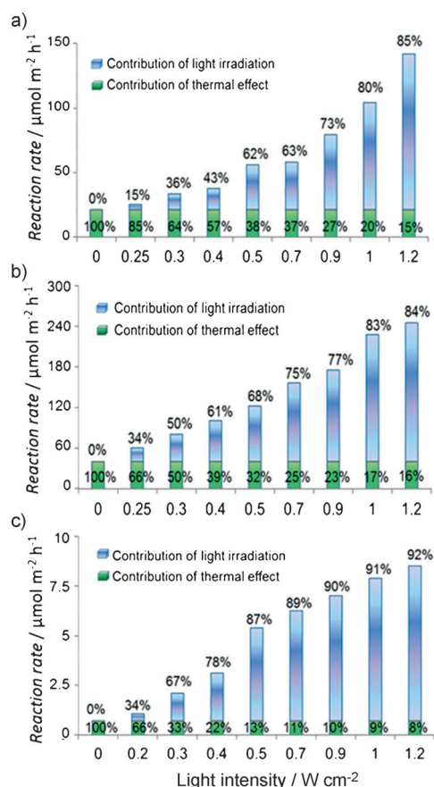
Figure 3. Dependence of the contributions from light irradiation and the thermal effect on the light intensity: a) dehydrogenation of benzyl alcohol to benzaldehyde on Pd@ZrO 2 at 45°C; b) degradation of phenol with Pt@ZrO 2 at 30°C; c) oxidation coupling of benzylamine on Rh@ZrO 2 at 50°C. The temperature of the reaction was maintained at the designated temperature when the irradiance was changed. The contribution due to light irradiation to the reaction rate was calculated by subtracting the rate of the reaction in the dark (performed at the same temperature) from the rate under light irradiation. The relative contributions of light irradiation and thermal catalysis to the reaction rate could then be determined.
